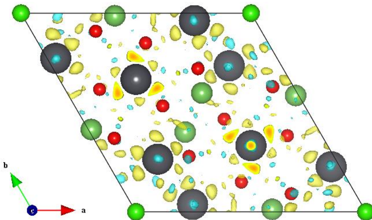
Figure S3. Three dimensional difference Fourier map from the X-ray diffraction data for finnemanite collected at 100K. The regions of electron density > 4 electrons (max. 9.5 electrons) are shown in yellow/orange.
